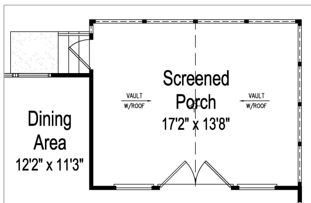
Screened Porch Option
